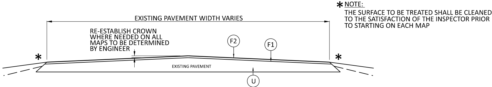
TYPICAL SECTION NO. 1
