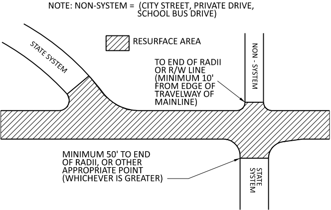
PAVING DETAIL 1 MAIN LINE IS BEING RESURFACED
